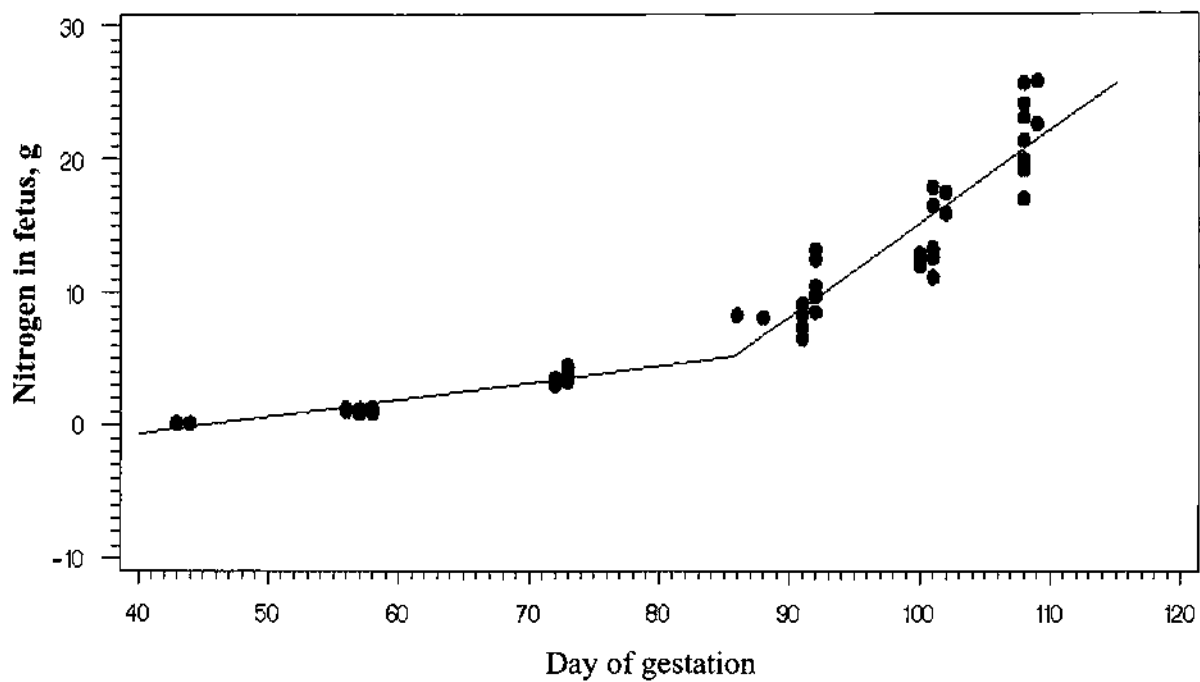
Figure 2. Fetal nitrogen broken-line analysis from d 43 to 108 of gestation ( n = 65 litters). Breakpoint of the nitrogen in fetus (g) occurred at d 85.8 of gestation ( R^2 = 0.95 , P < 0.01 ), showing that fetal nitrogen accretion mainly occurred after d 85.8 of gestation; the regression equation before d 85.8 was: 0.1263 \times (d - 85.8) + 5.1865 . After d 85.8 the equation was: 0.7007 \times (d - 85.8) + 5.1865 , where d is day of gestation.
